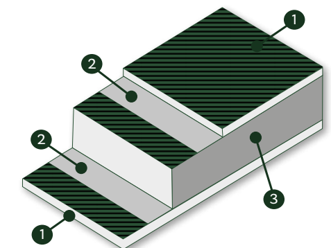
▲ Cross-section aluminium composite panel 1. aluminium top layer 2. adhesive layer 3. fire-retardant plastic core
